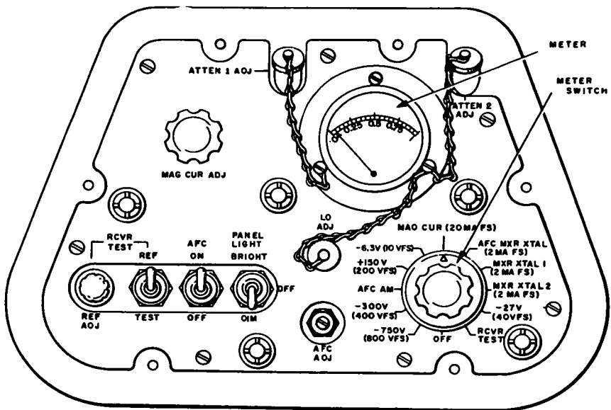
Figure 5. Receiver-transmitter meter panel.
