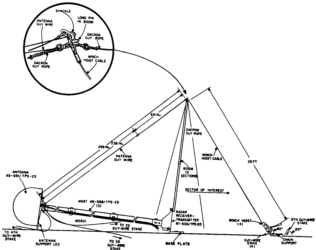
Figure 4. Layout of antenna for erection.
