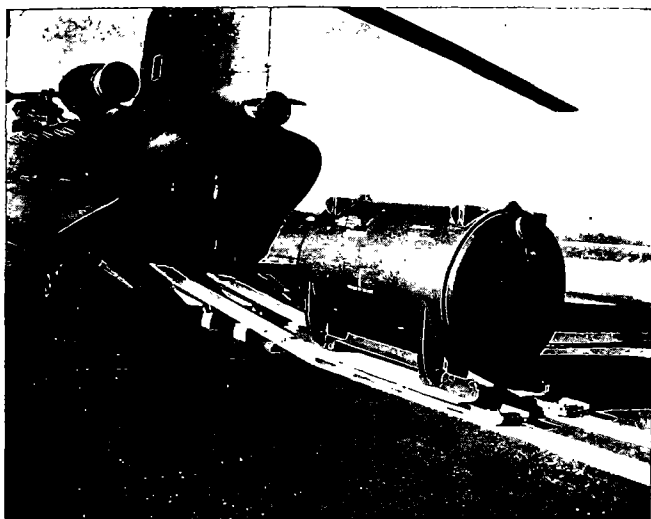
Figure 3-1. Shipping and storage container, M409, for Nike-Hercules warhead section. Container is positioned for loading into CH-47 helicopter.
