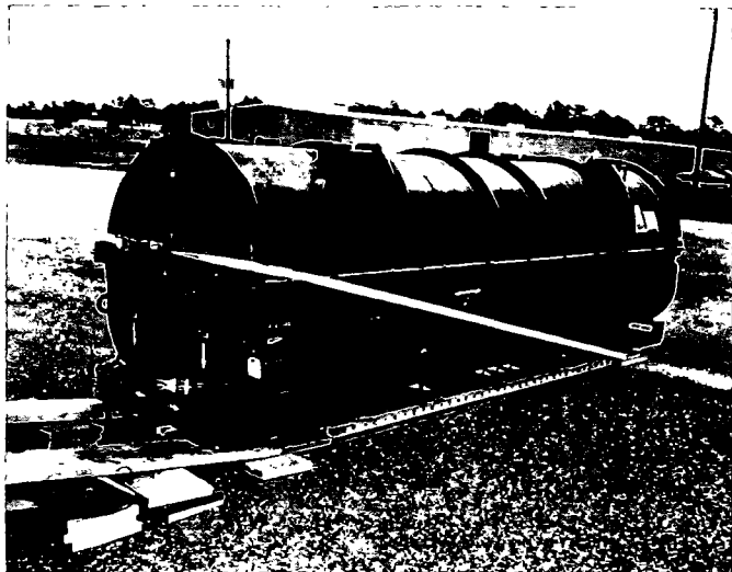
Figure 4-3. Placement of CGU-1/B tiedown devices to restrain container during loading. Shown is the M483 container for Pershing warhead section.
